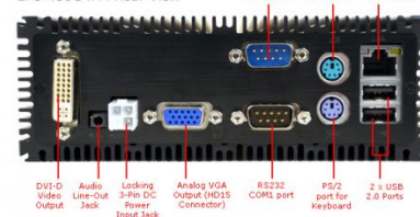
LPC-480G4FM Rear View
