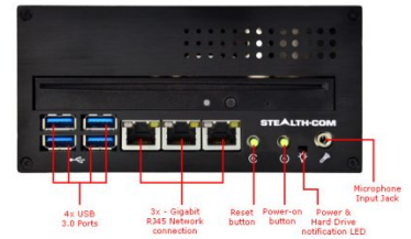
LPC-480PCleG4 Front View
