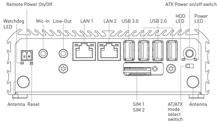
Front Panel
