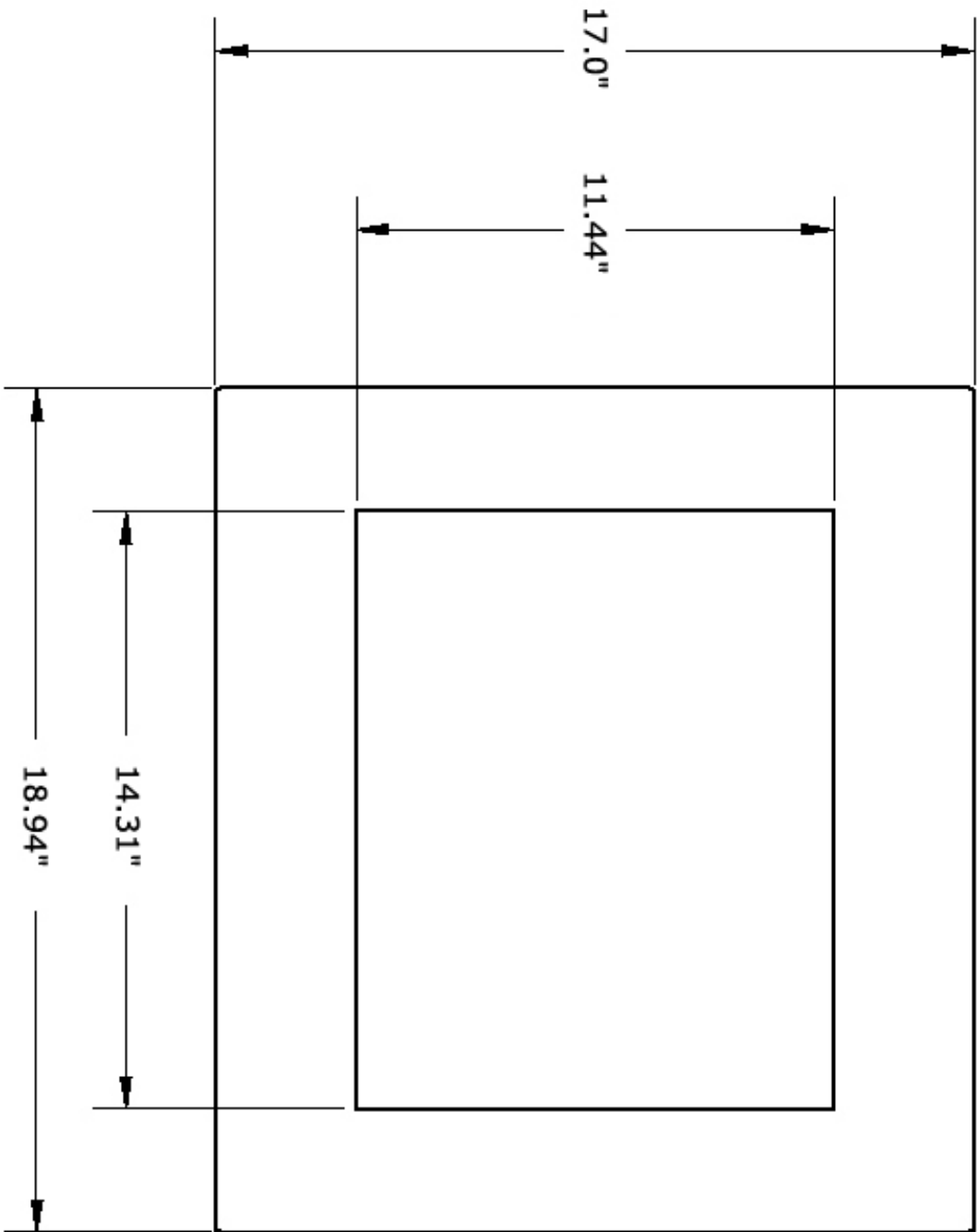
FRONT VIEW
