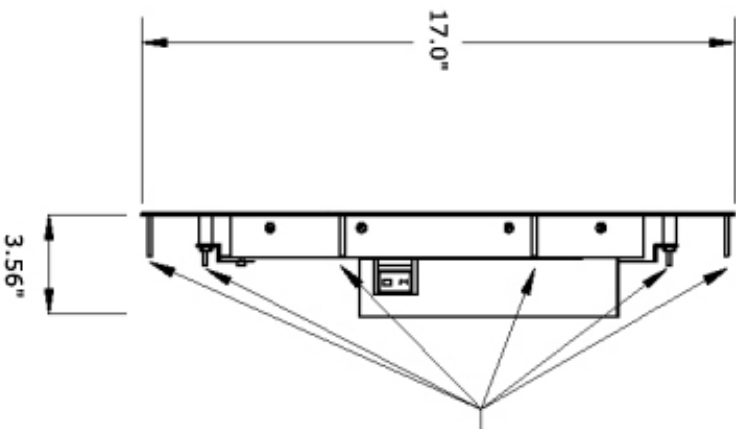
MOUNTING STUDS
