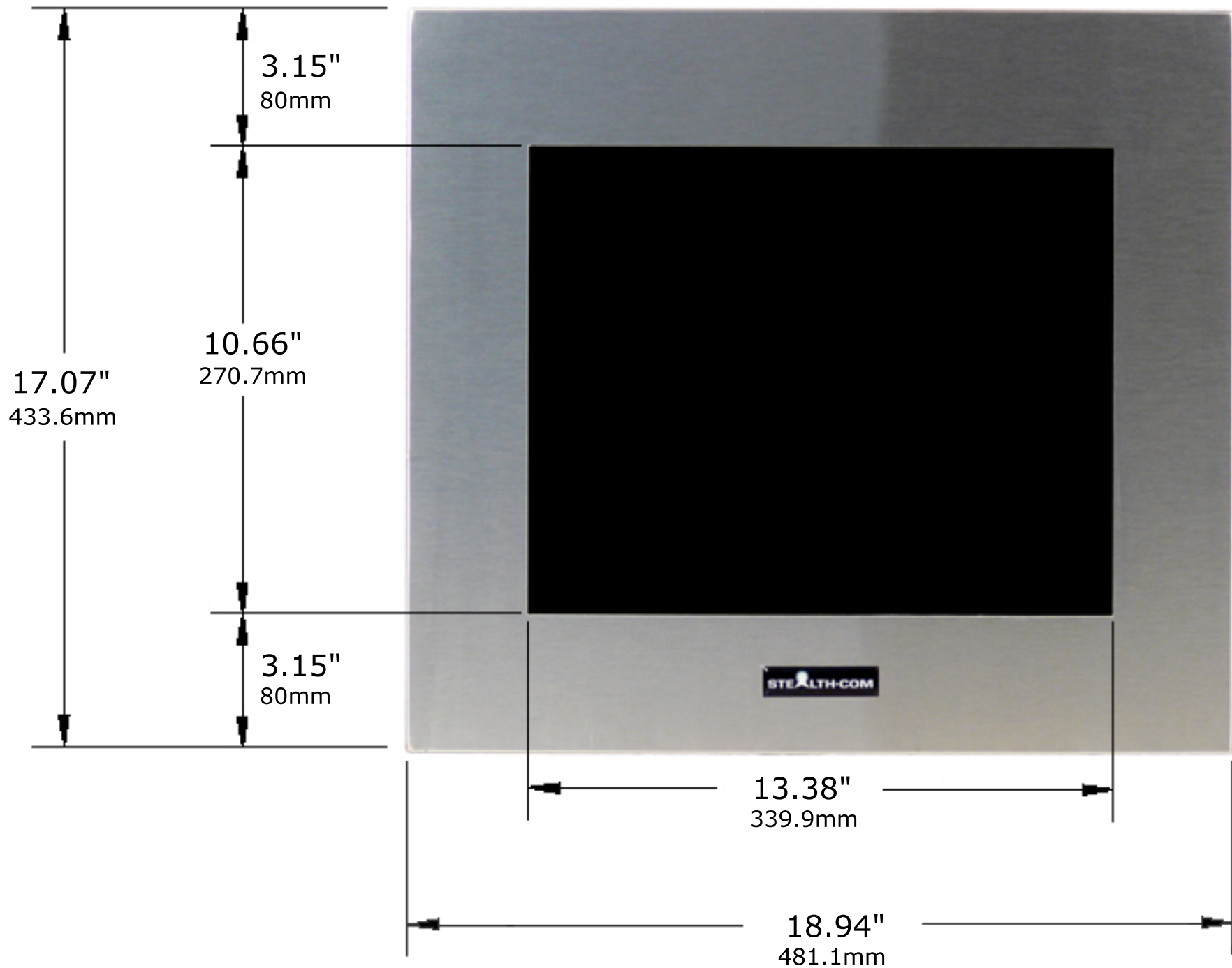
FRONT VIEW
