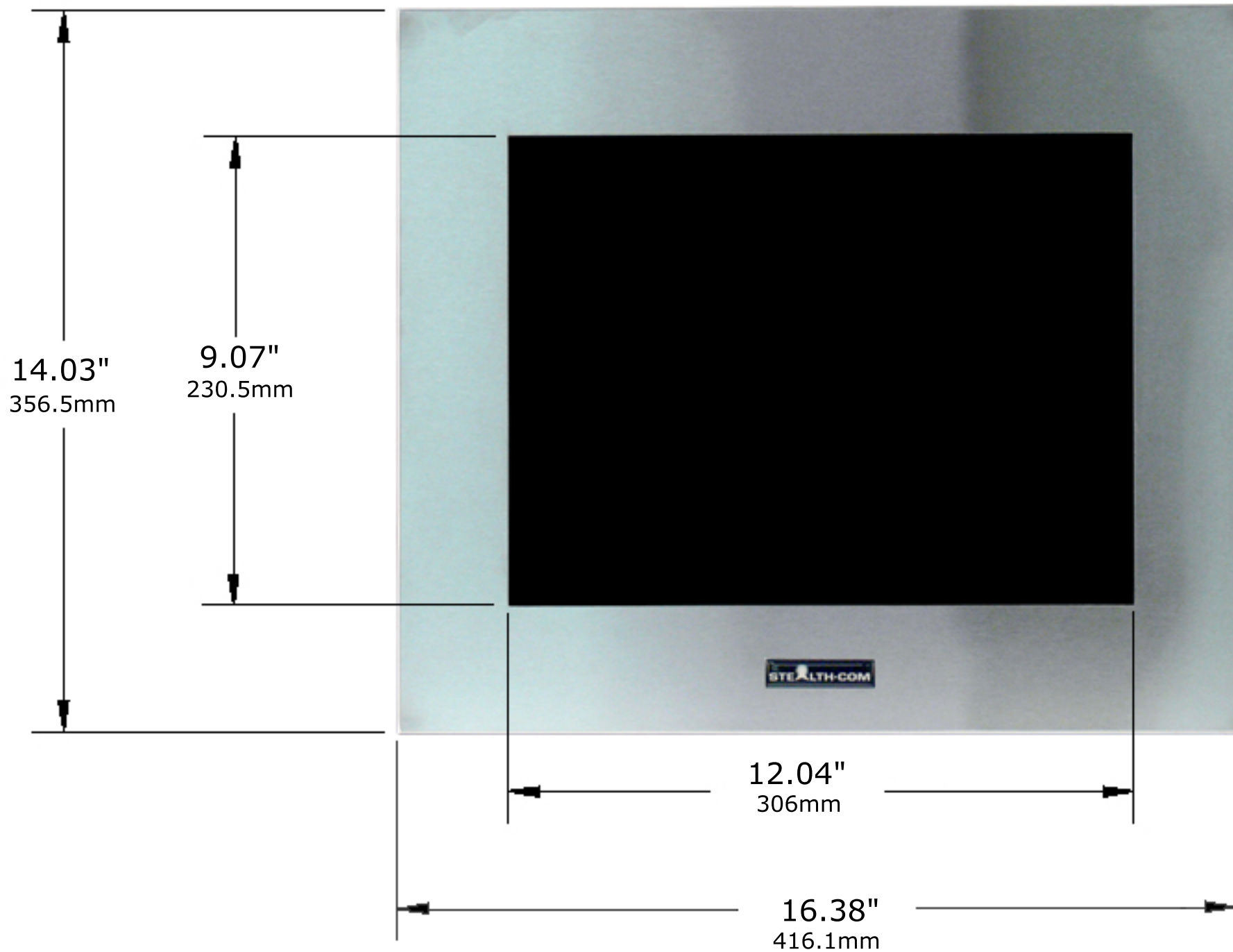
FRONT VIEW
