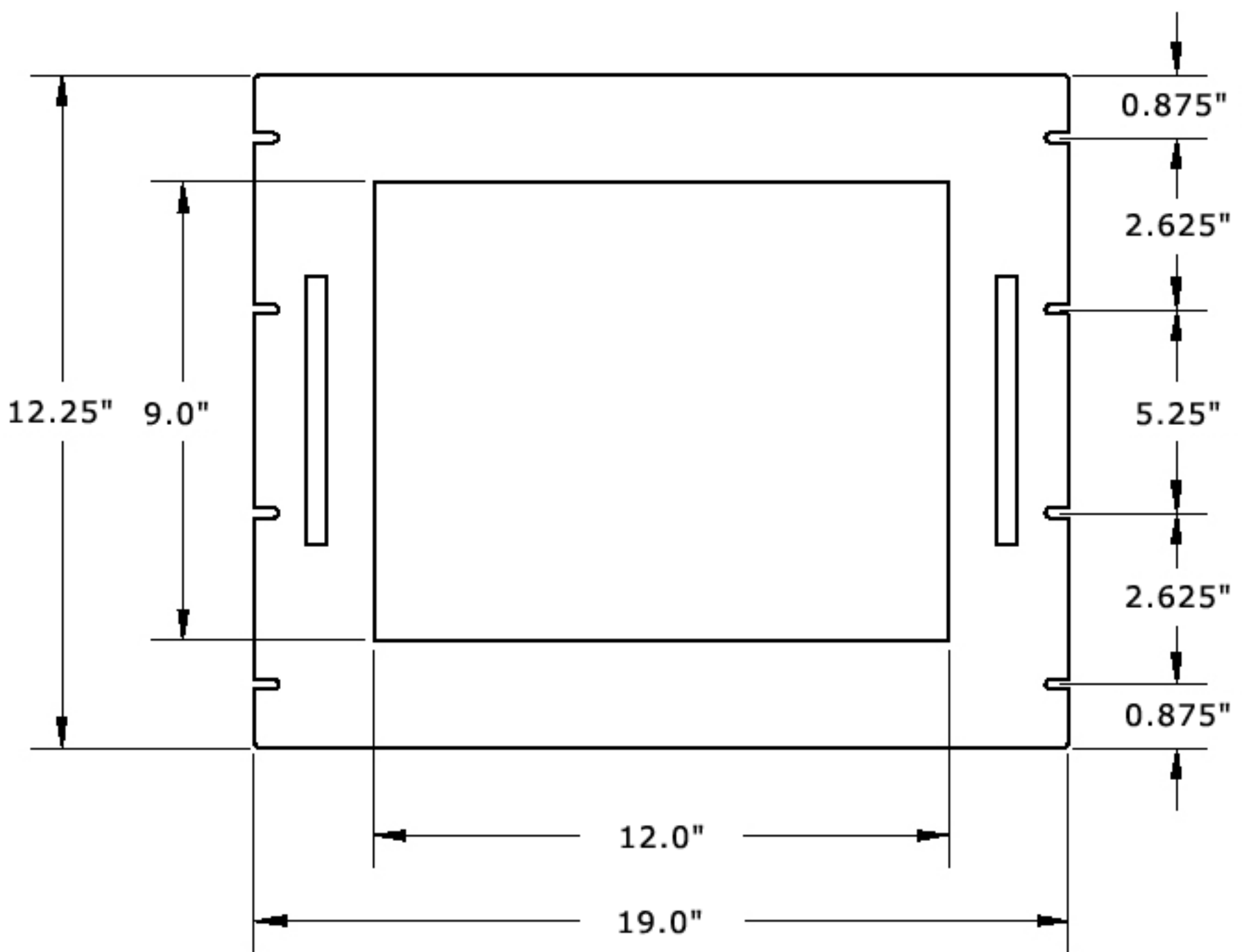
FRONT VIEW
