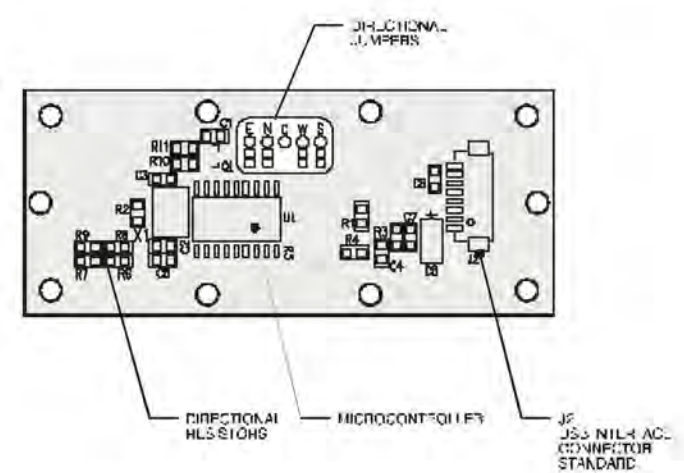
Rear - USB
