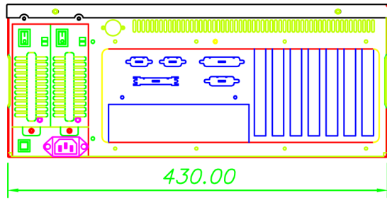
Rear view
