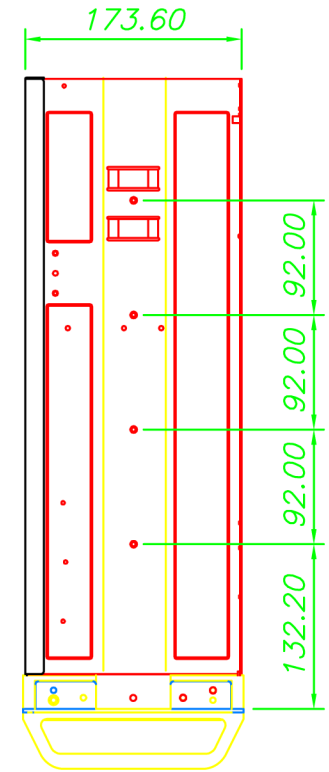
Right-side View
