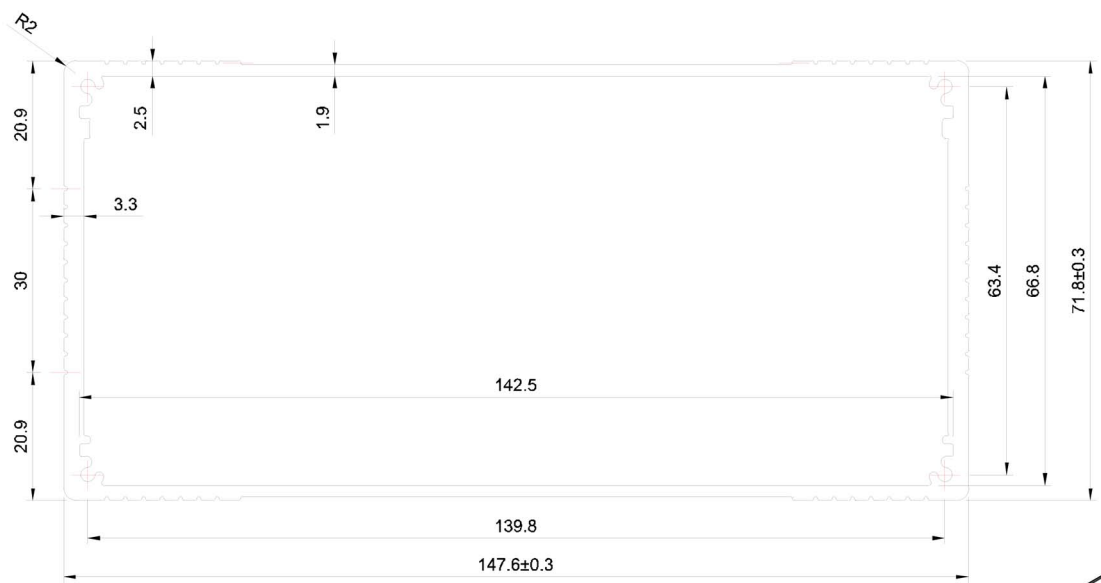
LPC-450PCI/LPC-460PCI chassis sectional drawing
